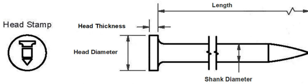
FIGURE 1—AEROSMITH SUREPIN® SMOOTH SERIES FASTENERS
