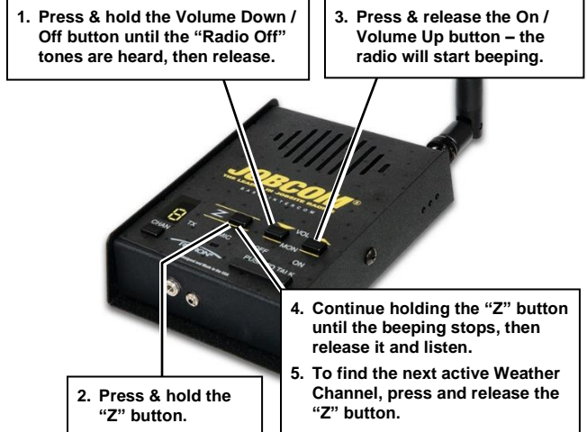
FIG-5: SELECTING YOUR LOCAL NOAA WEATHER FREQUENCY
