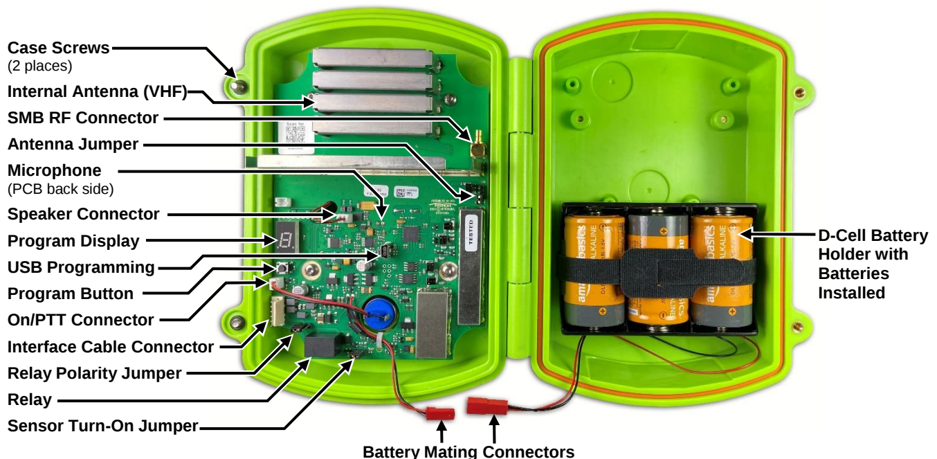
FIG-2: Callbox Assembly, Controls and Connectors
