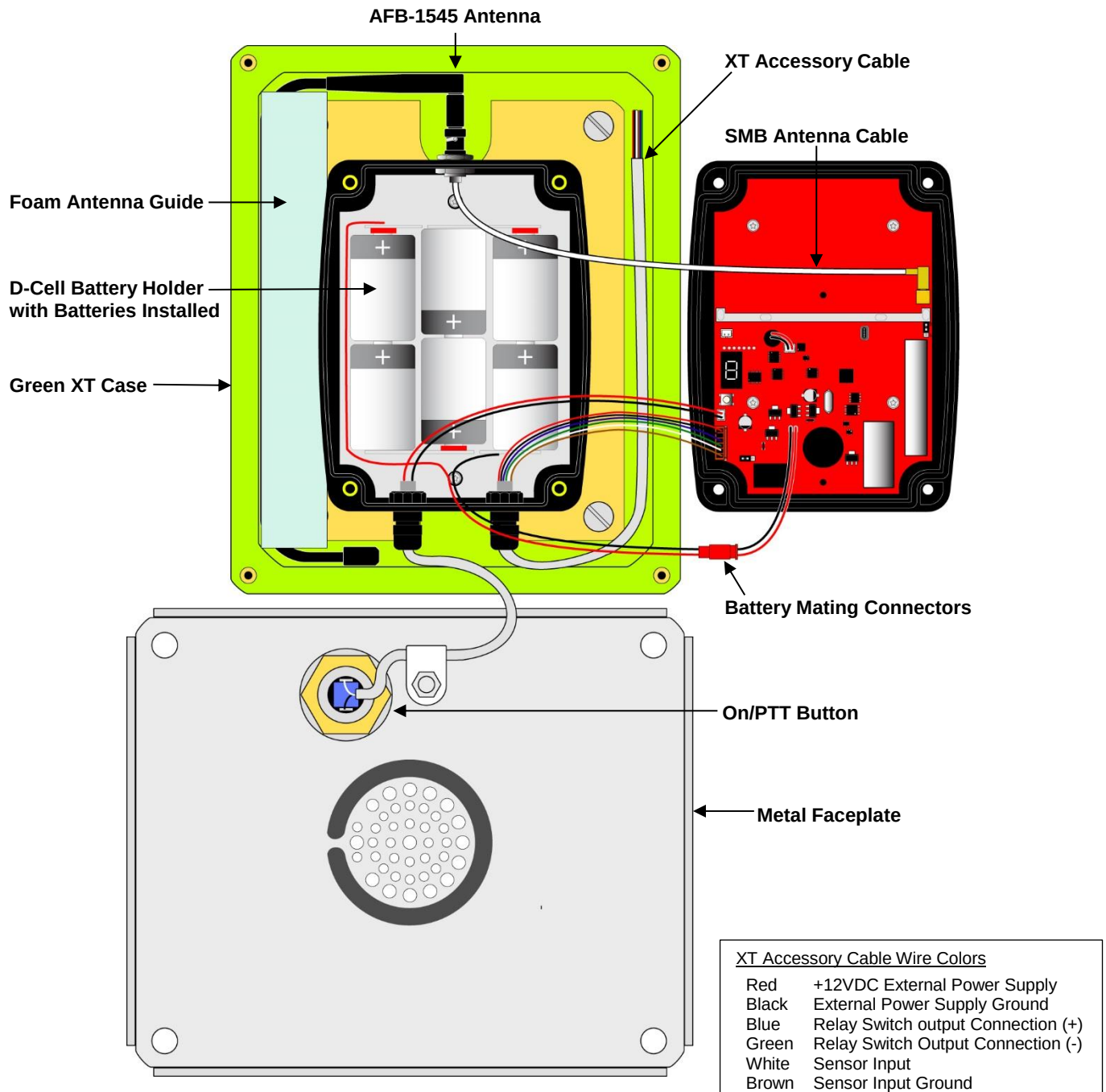
FIG-3: XT Callbox Assembly
