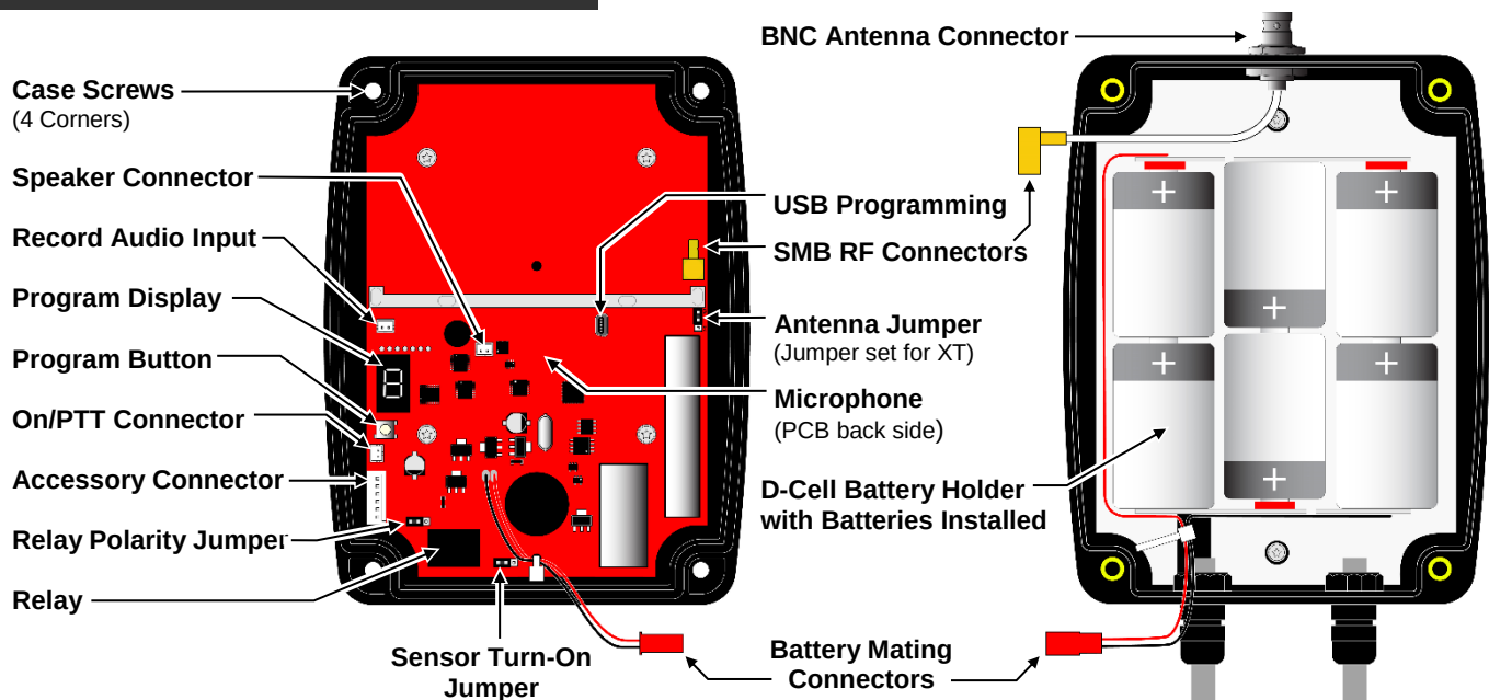
FIG-2: XT Callbox Controls and Connectors
