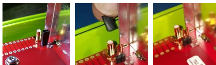
Antenna Jumper installed for use with built-in antenna
