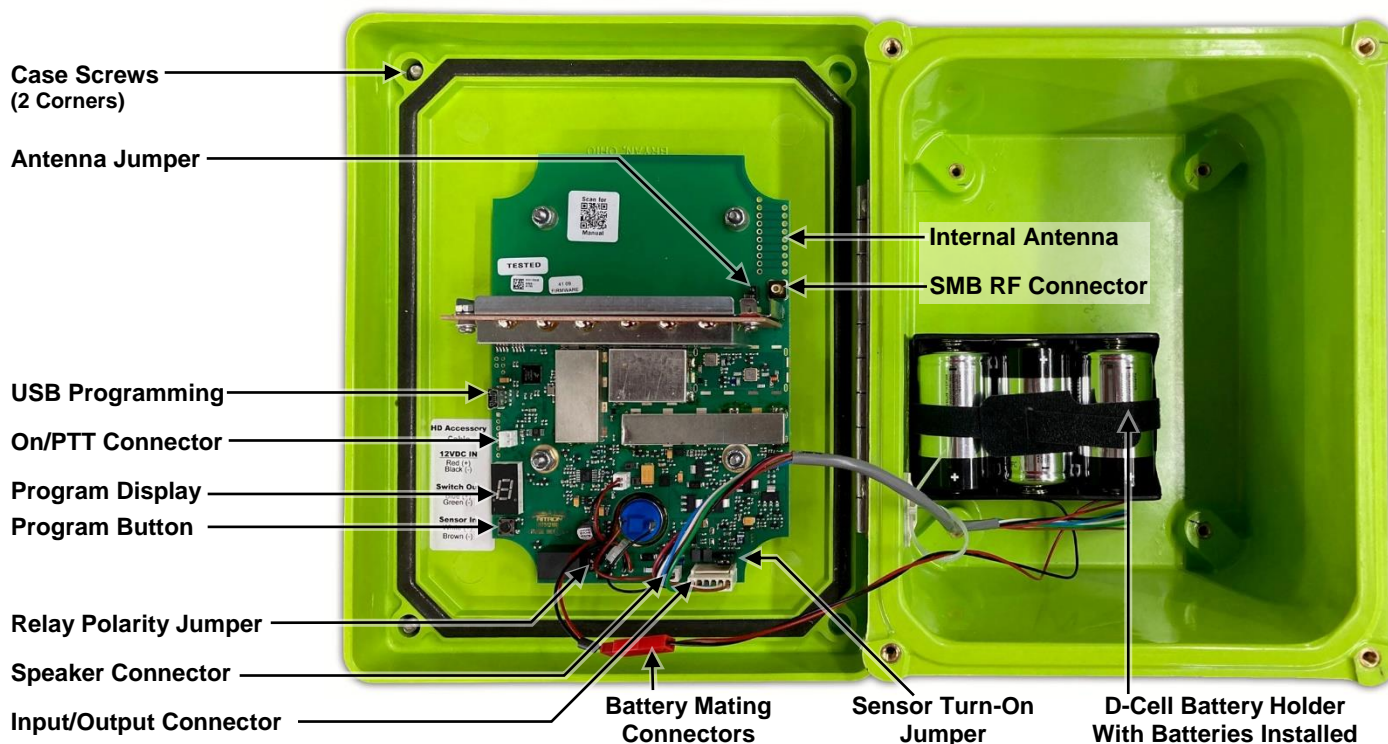
FIG-2: Callbox Assembly, Controls and Connectors
