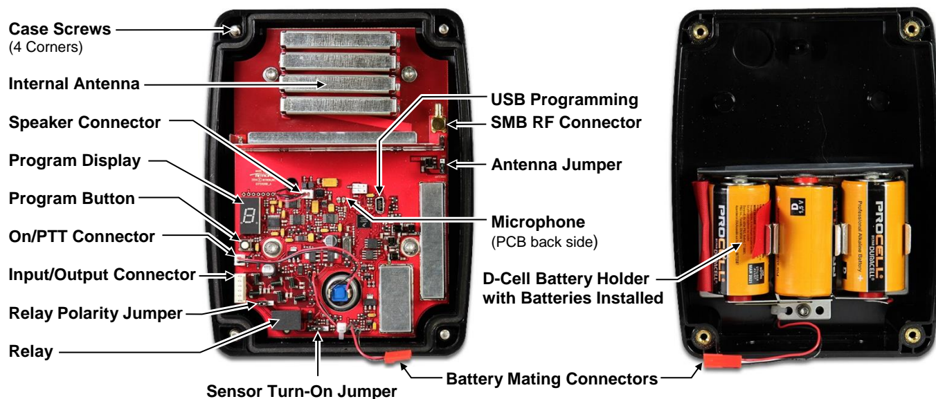
FIG-2: Callbox Assembly, Controls and Connectors
