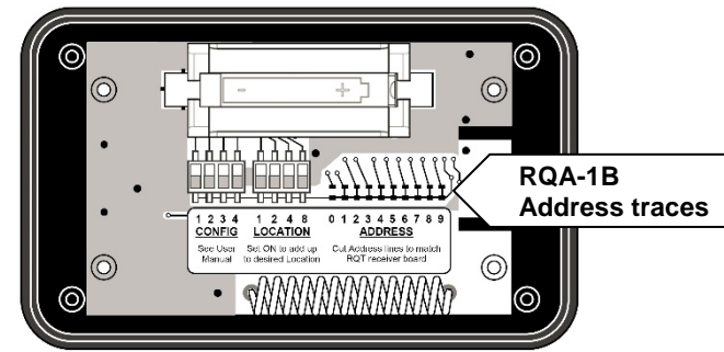
RQA-1B Address Programming
