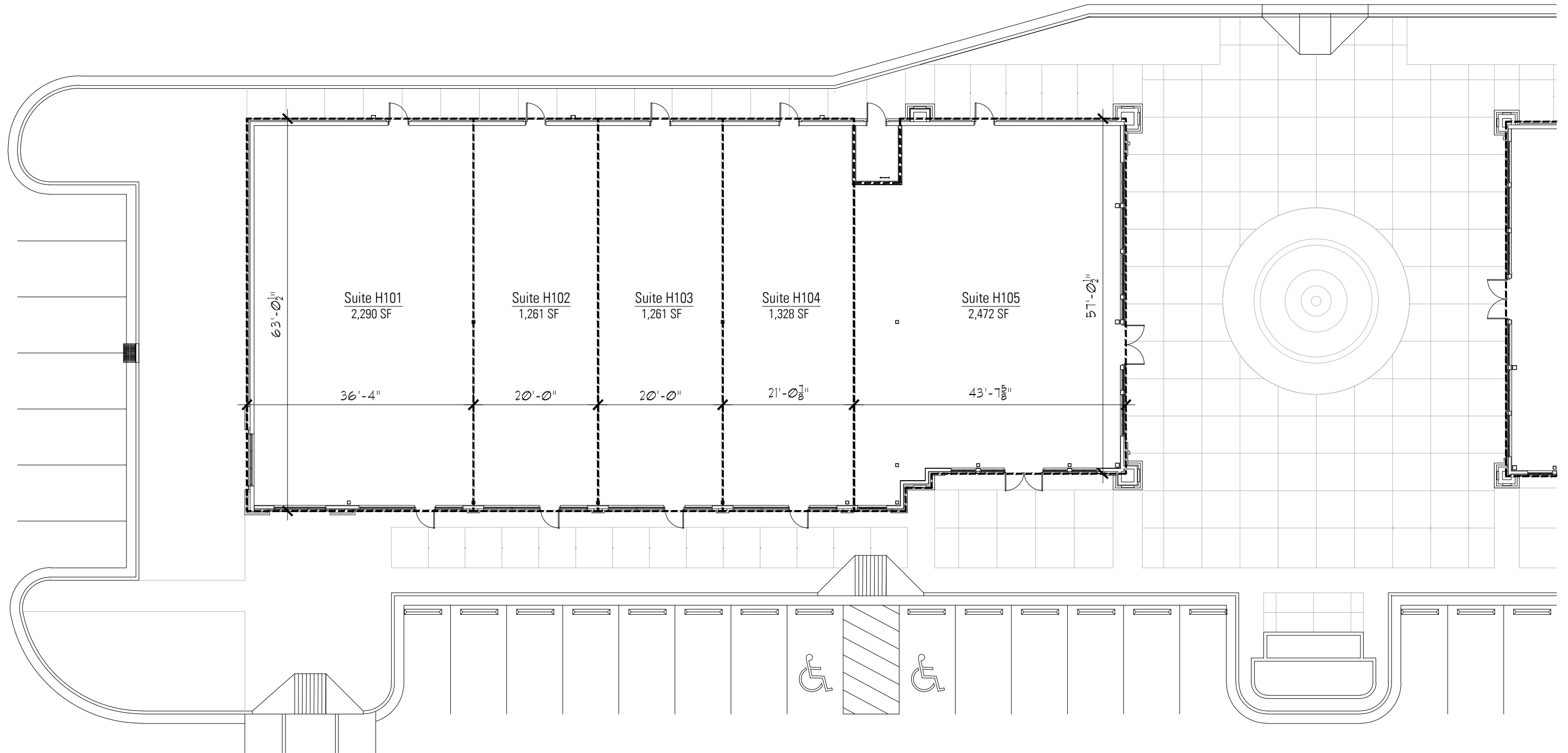
FLOOR PLAN Scale 1/16" = 1'-0"
