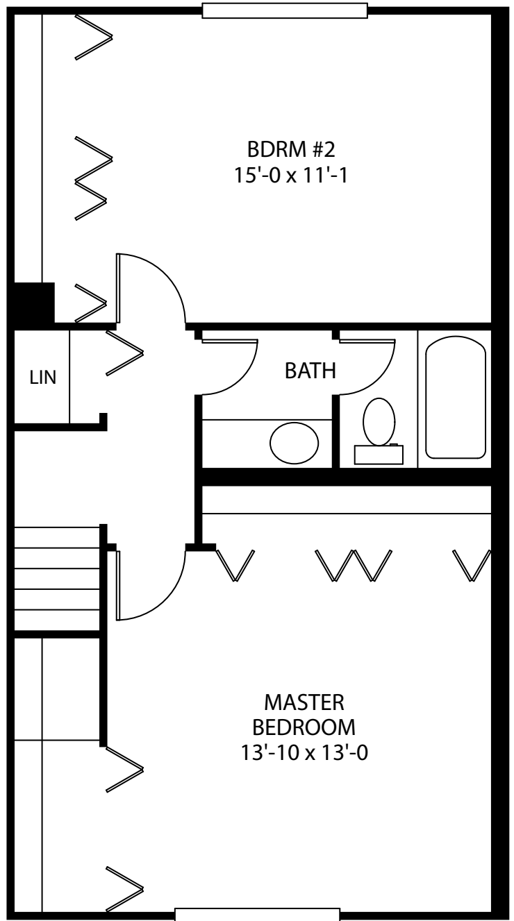
SECOND FLOOR
