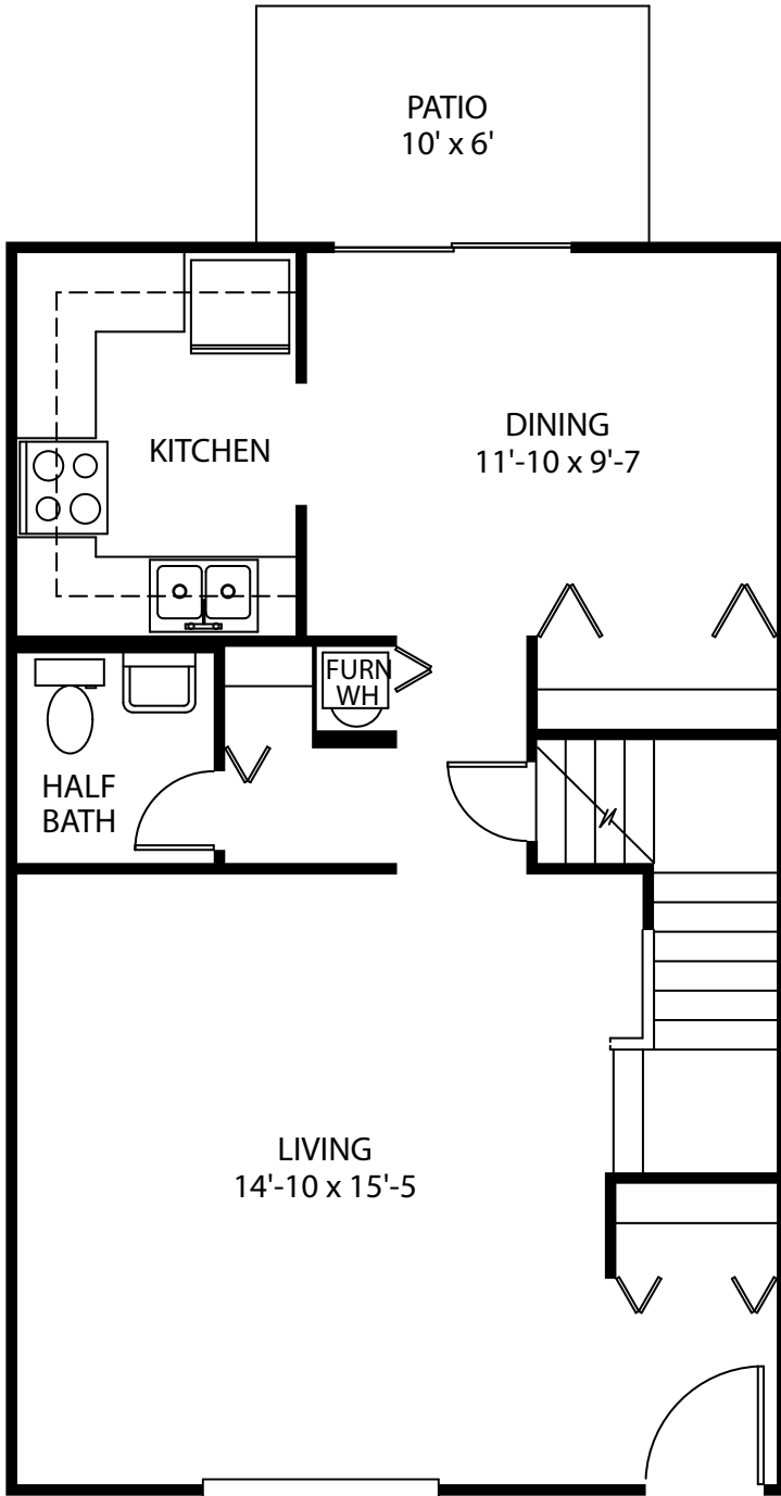
FIRST FLOOR
