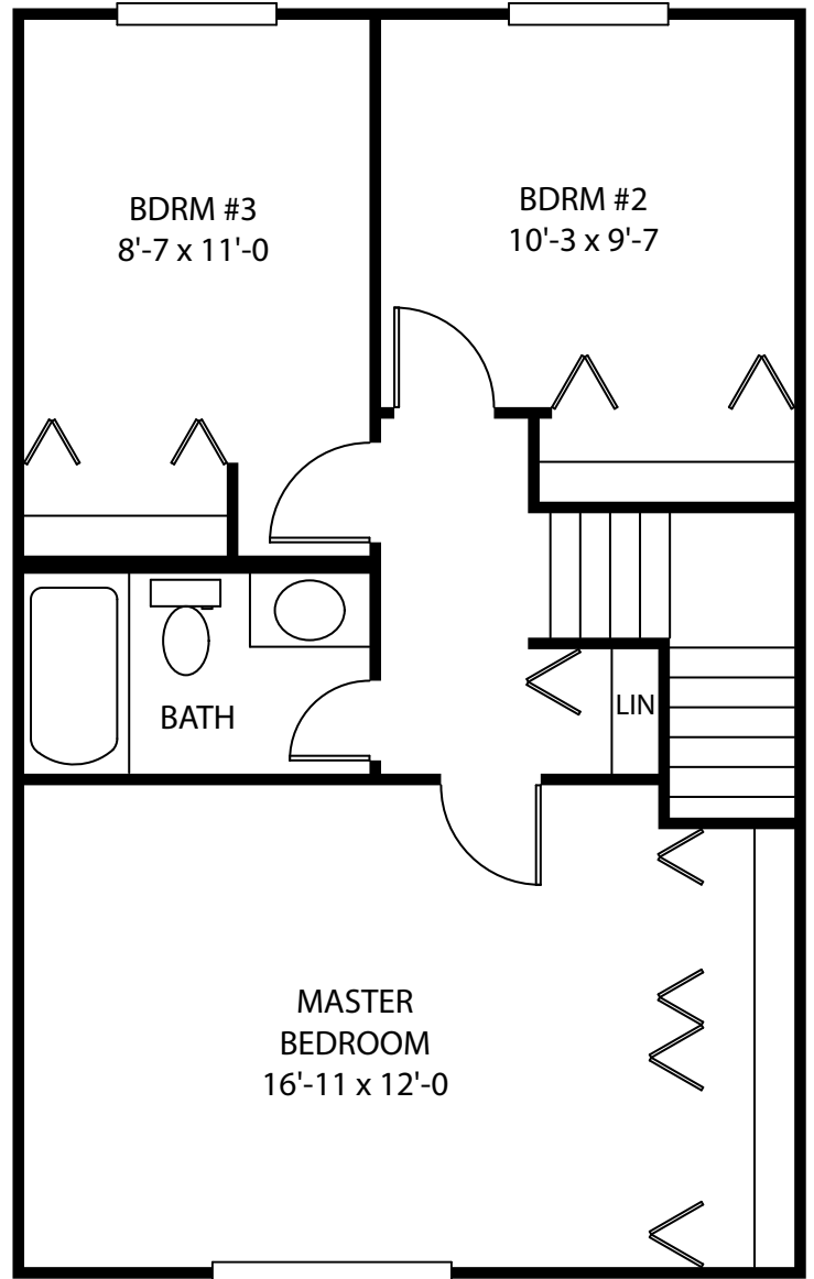
SECOND FLOOR
